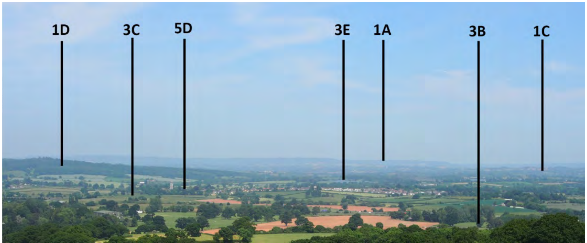
View east from Pinhoe, north of Exeter, showing how LCTs relate to each other
